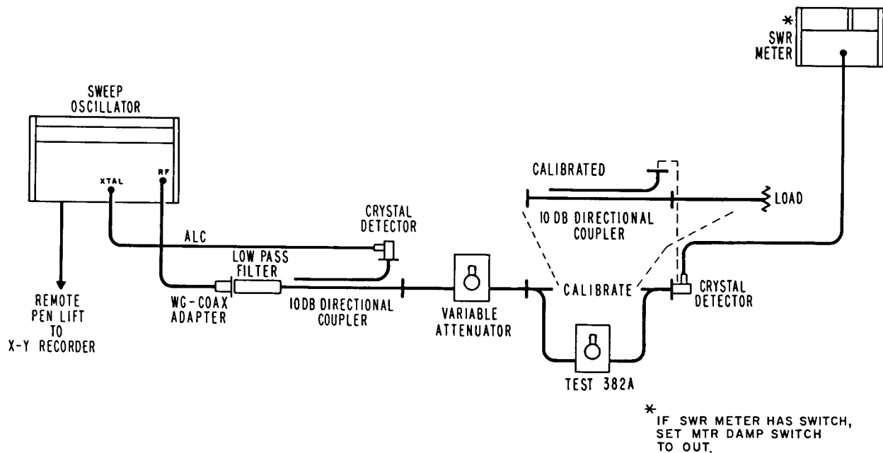
Figure 6 Attenuator Calibration
