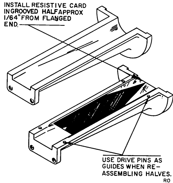
Figure 12 Installation of Resistive Card in End Section
