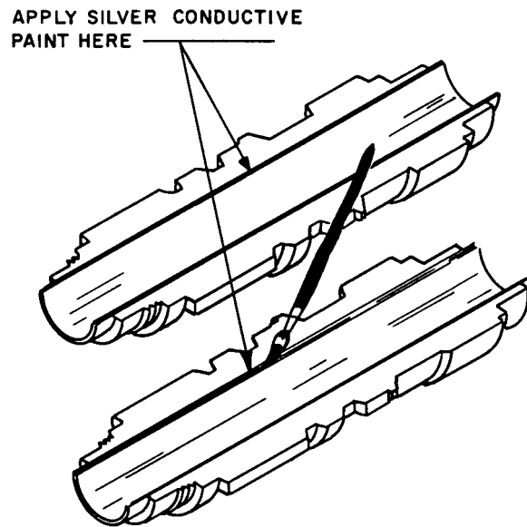
Figure 9 Application of Conductive Silver Paint to Center Section
