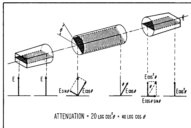
Figure 1 Attenuation Principle
